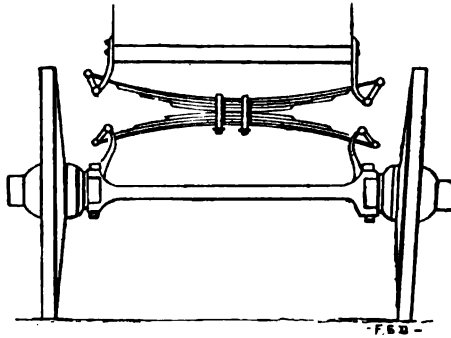
FIG. 77.—Forward Axle of the Jeanteand Electric Carriage, showing double half elliptic springs with connections by links to frame and body.
